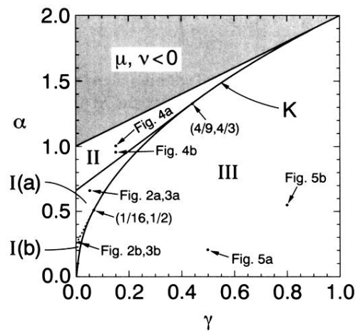
FIG. 6. Regions of the (\gamma, \alpha) parameter space (unshaded) corresponding to physical systems with positive friction.
