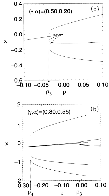
FIG. 5. (a) Bifurcation diagram for (\gamma, \alpha) = (0.50, 0.20) and \tau^2 = 1 . A stable period-3 maximal orbit and an unstable period-3 maximal orbit are simultaneously created in a saddle-node bifurcation at \rho = \rho_3 < 0 . The dashed curves indicate the locations of the unstable period-3 orbit. The stable period-1 orbit and the stable period-3 orbit are on the solid curves. One can see that the unstable period-3 orbit collapses onto the stable period-1 orbit at \rho = 0 . (b) Bifurcation diagram for (\gamma, \alpha) = (0.80, 0.55) and \tau^2 = 1 . A pair of stable and unstable period-3 maximal orbits are created in a saddle-node bifurcation at \rho = \rho_3 < 0 , and a pair of stable and unstable period-4 maximal orbits are created in a saddle-node bifurcation at \rho = \rho_4 < 0 . The unstable periodic orbits are not shown.
